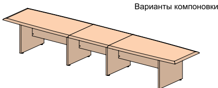
63S004 + 63B003 + 63B004 4800x1000x748
